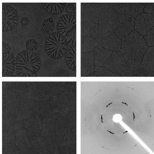
Figure 2. Homeotropic growth of 6 between ITO-coated glass slides as seen by polarized optical microscopy (slightly uncrossed polarizers, contrast enhanced, 0.2 mm × 0.2 mm): upper left: at cooling through liquid-to-LC phase transition; upper right: at slightly lower temperature; lower left: at 100 °C. Lower right: X-ray diffraction pattern of a homeotropically oriented sample taken at room temperature between thin glass slides: several domains of slightly different orientations of the hexagonal column lattice in the sample plane are diffracted simultaneously, as the beam width covers more than one domain.
