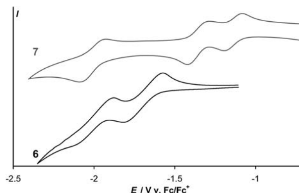
Figure 4. Cyclic voltammetry on 1 mM solutions of 6 and 7 in 0.1 M solutions of \text{Bu}_4\text{NPF}_6 in dichloromethane. Scan rate: 0.1 \text{Vs}^{-1} .
